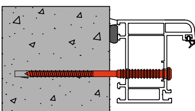
PVC frame - Concrete support
