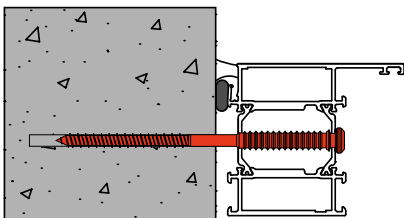
Aluminum frame - Concrete support
