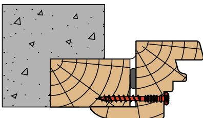
Wood frame - Wood support
