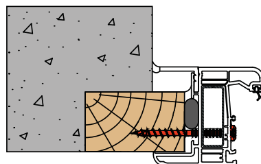
Steel Reinforced PVC frame - Wood Support
