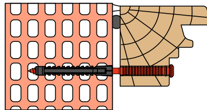
Wooden frame - Brick support
