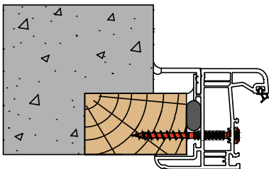
PVC frame - Wood support
