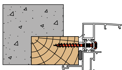
Aluminum frame - Wood Support
