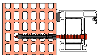
Reinforced PVC frame - Brick support
