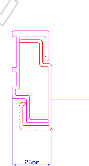
ASSEMBLY DIM
